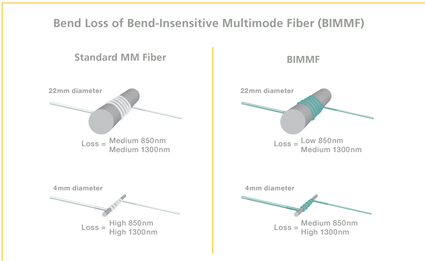
Figure 1: Bend Loss of Bend-Insensitive Multimode Fiber (BIMMF)
