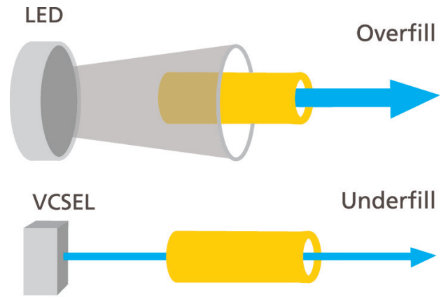
Two different fill conditions: Overfill (LED) and Underfill (VCSEL).
